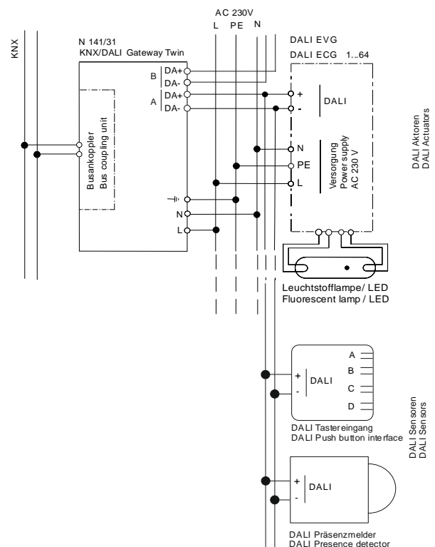
Fig. 2 Connection example for N 141/31
